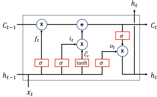
Fig. 11. LSTM cell overview. C_t , h_t , x_t , f_t , i_t , and o_t denote state of the cell, hidden state, input, output of forget gate, output of the input gate, and output of the output gate. C_{t-1} and h_{t-1} denote previous cell's state.
