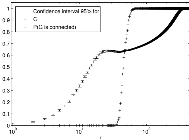
Figure 5. The effect on the clustering coefficient C and the probability P of a fully connected network when increasing transmission range r from 0 to the maximum.
