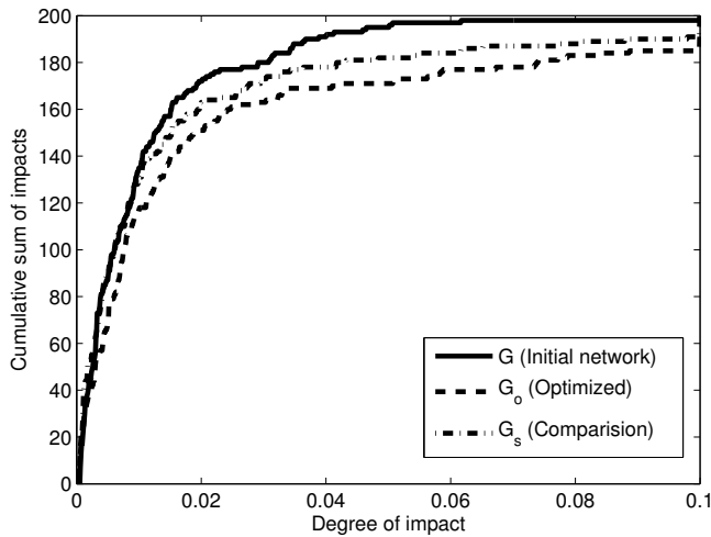
Figure 3. Test of robustness to failures with respect to the characteristic path length. The impact differences i , i_o and i_s are shown: the initial network G has been optimized by removing dedicated links and increasing C ( G_o ). A third network has been included into the graph, in which number of links corresponds to that of the optimized network ( G_s ).
