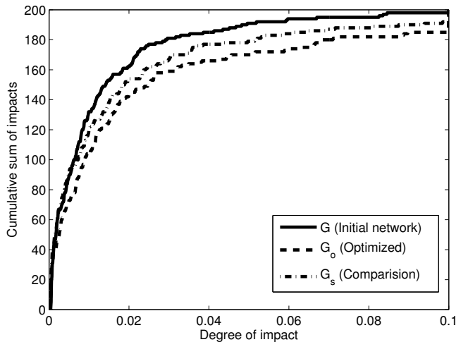
Figure 4. The test of robustness to attacks with respect to the characteristic path length. The impact differences i , i_o and i_s are shown: the initial network G has been optimized by removing dedicated links and increasing C ( G_o ). A third network has been included into the graph, in which number of links corresponds to that of the optimized network ( G_s ).
