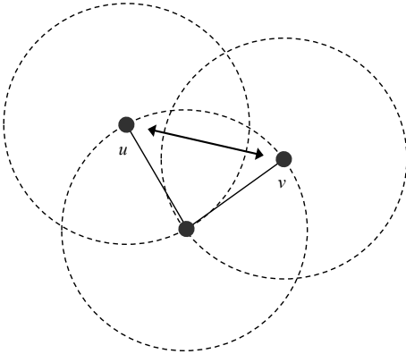
Figure 2. Increasing transmission establishes additional links, e.g. (u, v) .
